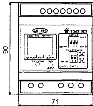
View and dimensions of synchronizer
